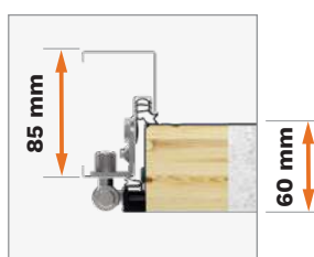
Ościeznica PERFOTHERM 60
